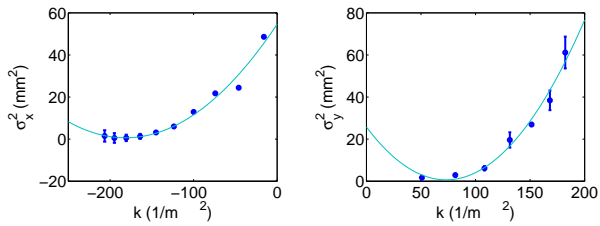
Figure 3: Squared horizontal (left) and vertical (right) beam sizes versus quadrupole magnetic strength. The data (blue circles) and corresponding quadratic fit (green lines) are shown. Emittance values inferred from the quadratic fit are \varepsilon_x = 18.5 \pm 2 \mu\text{m} and \varepsilon_y = 16.2 \pm 2 \mu\text{m} .
