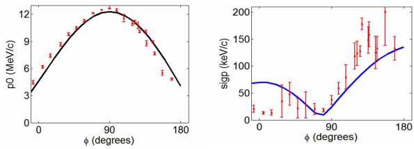
Figure 5: Mean (left) and rms (right) momentum versus booster phase. Red symbols are measurement and solid line are simulations with \varepsilon_z \simeq 8 \mu\text{m} .
