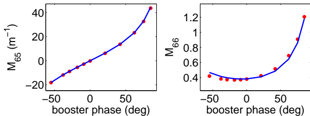
Figure 4: M_{65} (left) and M_{66} (right) element of the transfer matrix of the booster cavity in the longitudinal phase space (z, \delta) . The simulated transfer matrix using IMPACT-T (red symbols) is compared with analytical calculation (blue lines).
