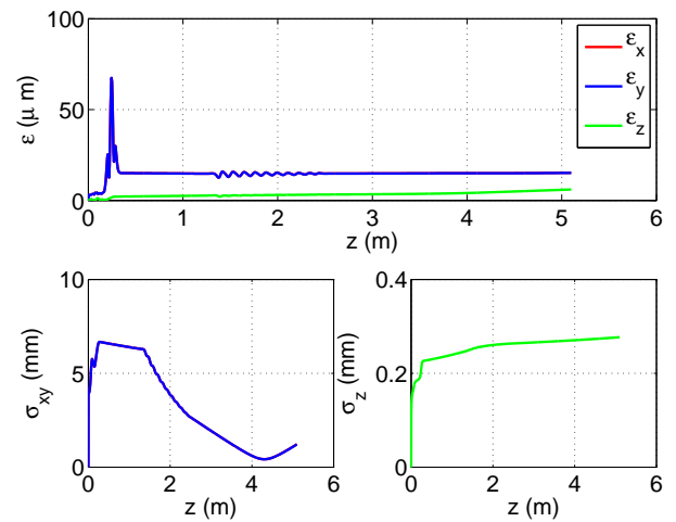
Figure 2: Top plot is the transverse emittance ( blue and red) and longitudinal emittance evolution along AWA beam line. Bottom plot is for the beam size and bunch length evolution.
